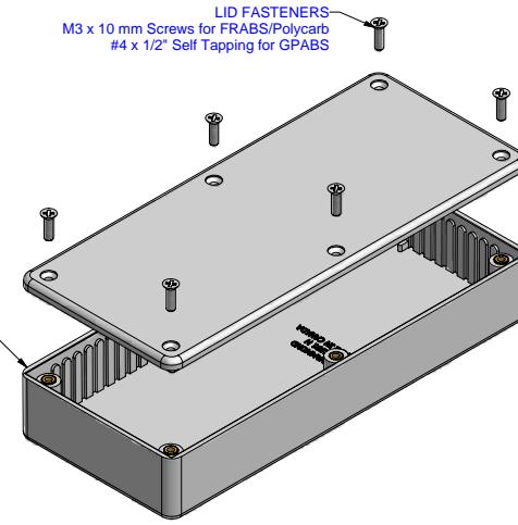
EXPLODED VIEW OF ASSEMBLY
